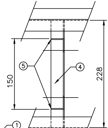
DETAIL 'Z'
